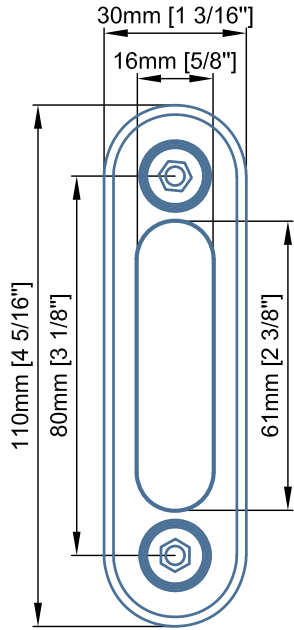
**Door Preparation / Drilling
